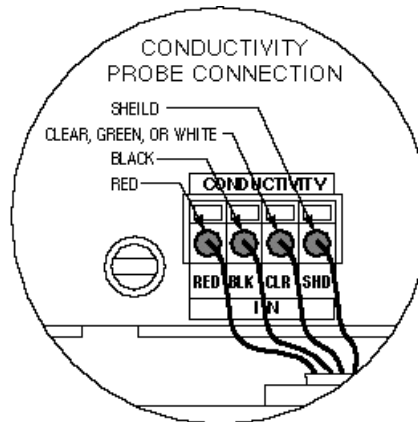
Fig. 4, Low Voltage Wiring Diagram
